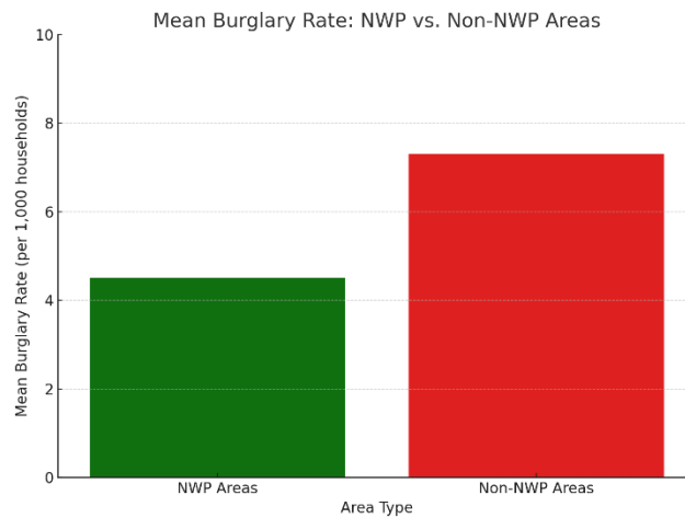
Figure 1. Results of Independent Samples t-test for Burglary Rates
